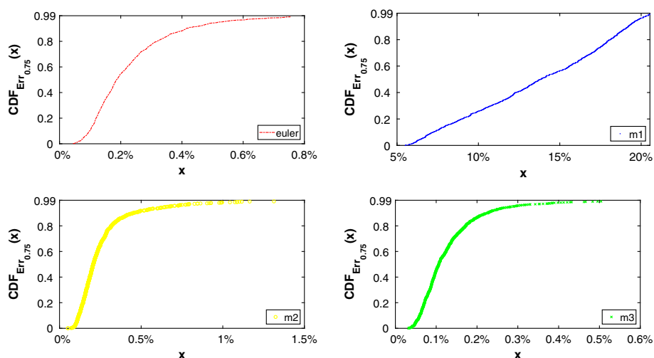
Fig. 5 B_t and A_t as in (56) normalized by its spectral norm. Empirical CDF of \text{Err}_t , at t = 0.75 , for euler, m1, m2, m3, with exact as benchmark solution, obtained with 10^3 samples
