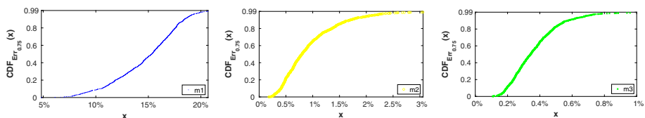
Fig. 2 A and B constant. Empirical CDF of \text{Err}_t , at t = 0.75 , for m1, m2, m3, with euler as benchmark solution, obtained with 10^3 samples
